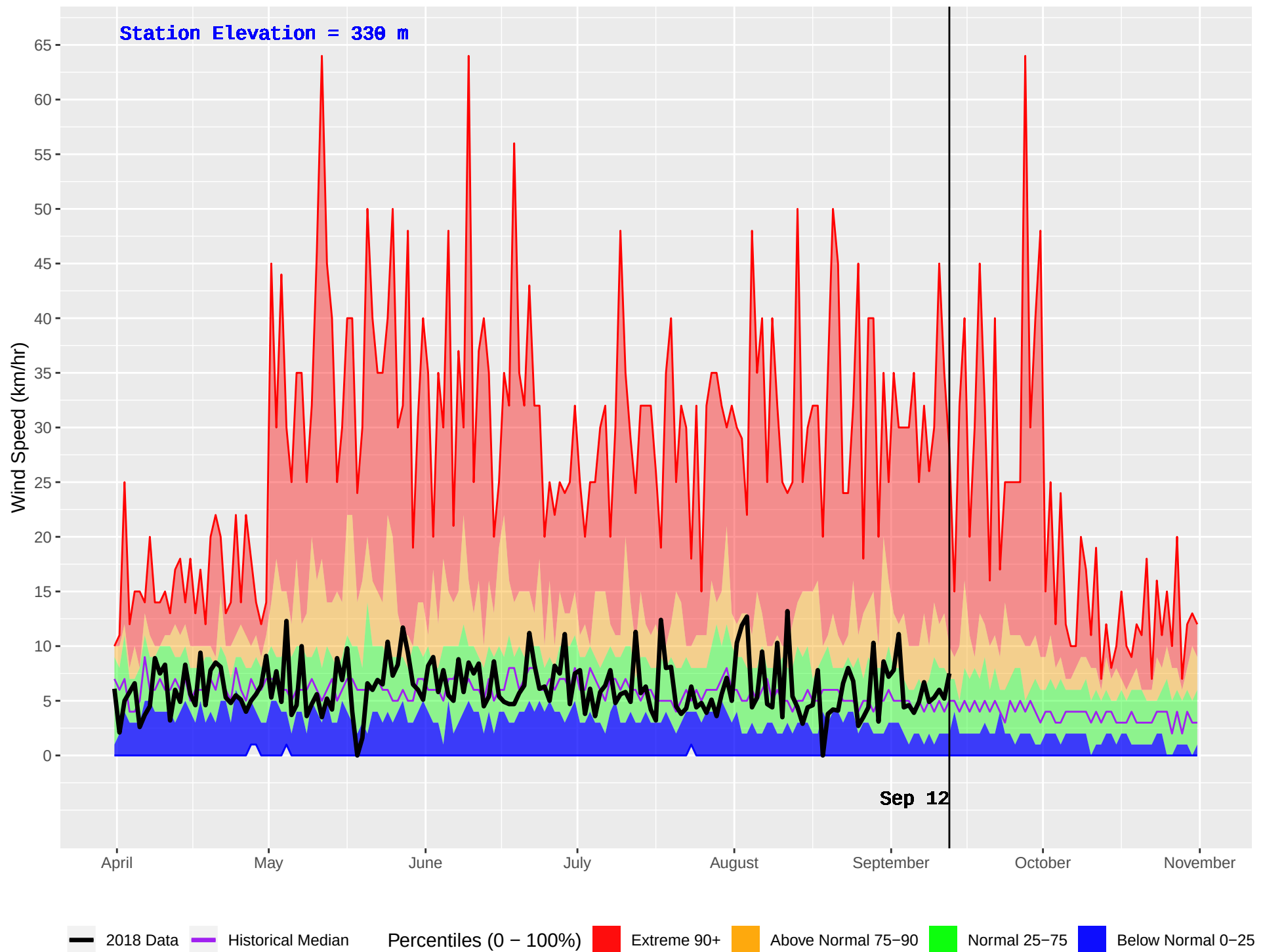
D'ARCY (292) : Historical (1978–2016) and Current (2018) Daily Wind Speed
