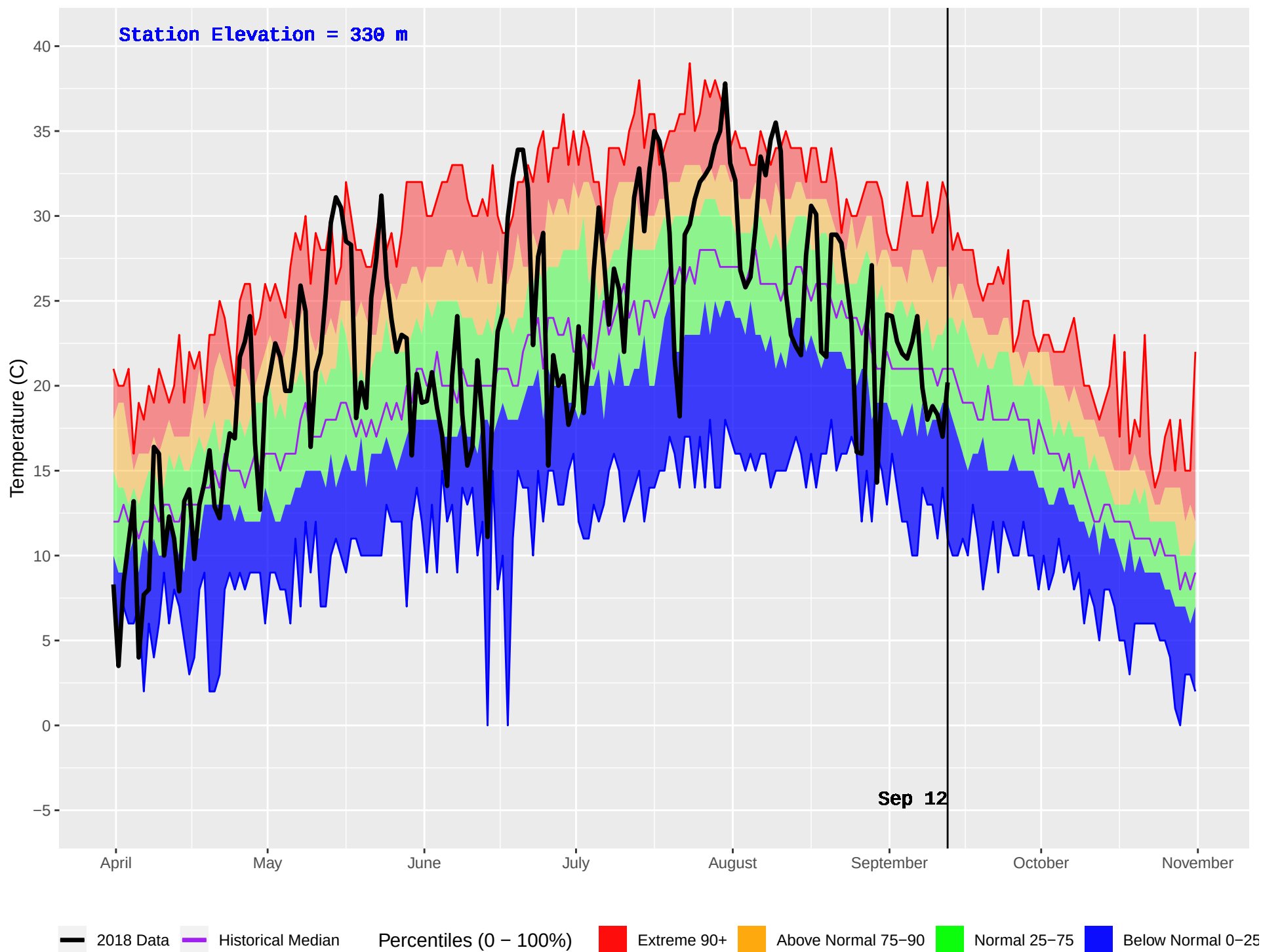
D'ARCY (292) : Historical (1978–2016) and Current (2018) Daily Temperature
